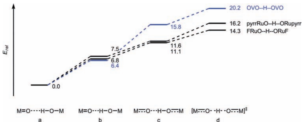
Figure 8. Relative gas-phase energies ( \Delta E in kcal mol -1 ) of (a) the optimized hydrogen-bonded precursor complexes ( E set equal to 0); (b) the O...O distances shortened to those in the transition structures, but all other geometrical parameters optimized; (c) all of the atoms moved to their positions in the transition structures, except for the transferring proton, whose position was optimized; and (d) the optimized transition structures.
