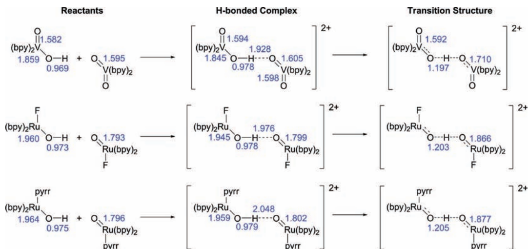
Figure 9. M=O, M-OH, and O-H bond lengths (Å) in the reactants, hydrogen-bonded complexes, and transition structures for three hydrogen atom self-exchange reactions.
