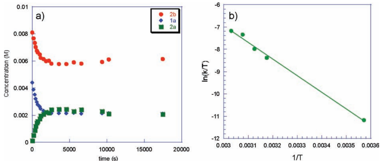
Figure 5. (a) Plot of the concentrations vs time for the pseudo-self-exchange reaction of 1a and 2b in \text{CD}_3\text{CN} at 320 K. (b) Eyring plot of pseudo-self-exchange rate constants.
