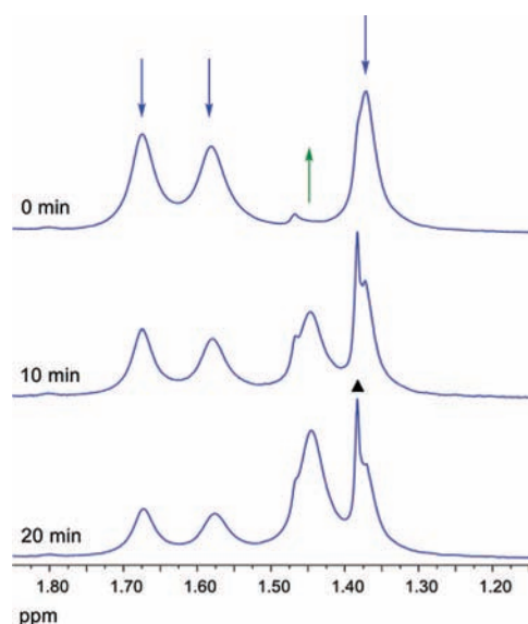
Figure 4. ^t\text{Bu} region of ^1\text{H} NMR spectra of the pseudo-self-exchange reaction between 1a and 2b at 320 K in \text{CD}_3\text{CN} ( \blacktriangle denotes free ^t\text{Bu}_2\text{bpy} ).
