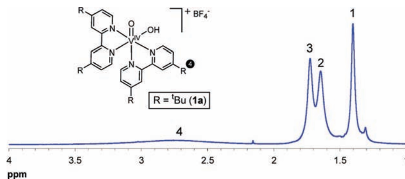
Figure 3. ^1\text{H} NMR of 1a in \text{CD}_2\text{Cl}_2 , with the ^t\text{Bu} peaks labeled 1–4.
