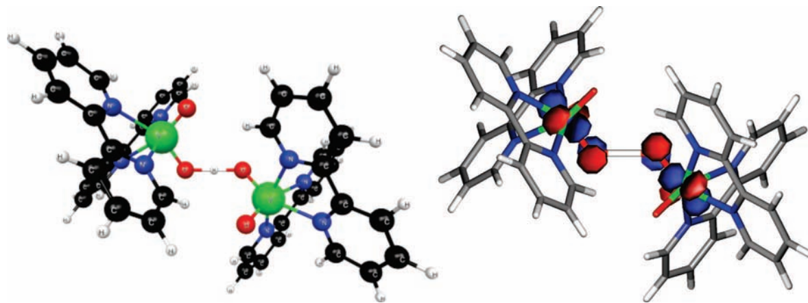
Figure 11. Computed structure (left) and SOMO (right) of the 1c + 2c transition structure. The V–O–O–V dihedral angle is 118.4°.
