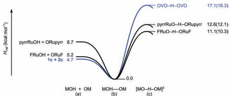
Figure 7. B3LYP/6-31G* PCM enthalpies ( \text{kcal mol}^{-1} ), relative to the hydrogen-bonded complexes (b), of the reactants (a) and transition structures (c) in three degenerate hydrogen-exchange reactions in acetonitrile solution. For the transition structures, the gas-phase enthalpies are given in parentheses.
